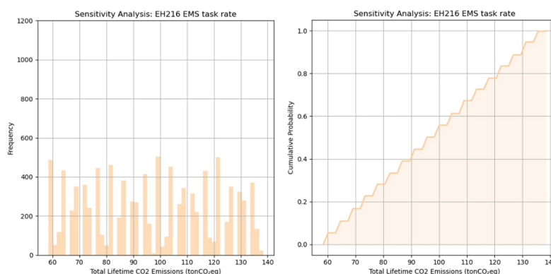
Figure 30: Sensitivity analysis: EH216 EMS task rate as the only variable (Helsinki)
