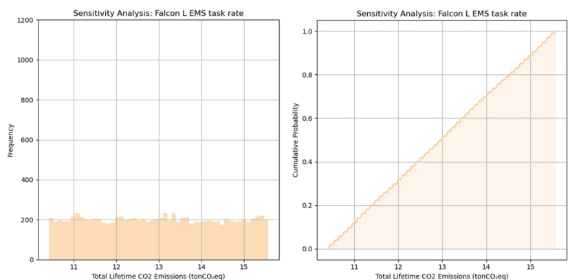
Figure 26 Sensitivity analysis: Falcon L EMS task rate as the only variable (Helsinki)
