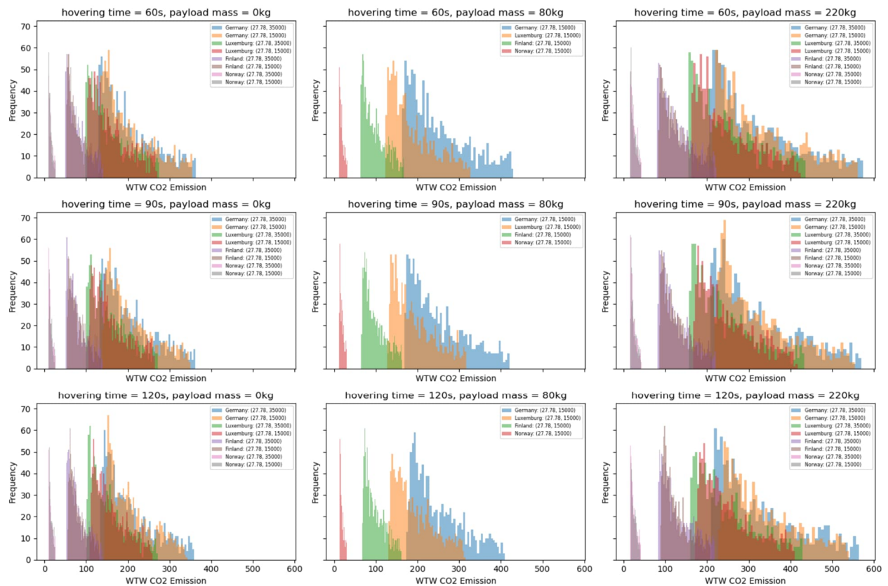
Figure 20 Frequency distribution of WTW CO 2 Emission values of EH216 for each combination of sensitivity analysis variables
