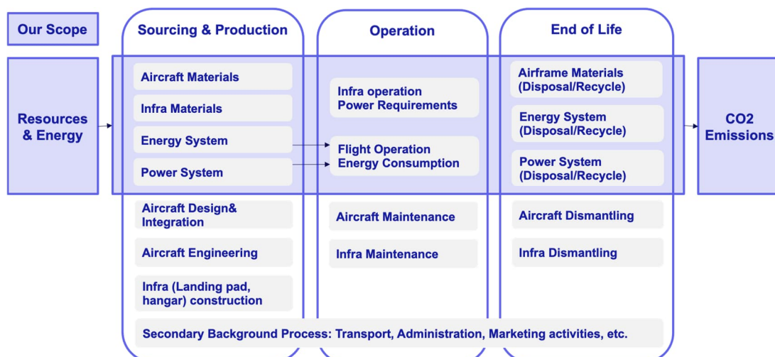
Figure 10: Life cycle stages and inventories of UAS (André, 2022)
