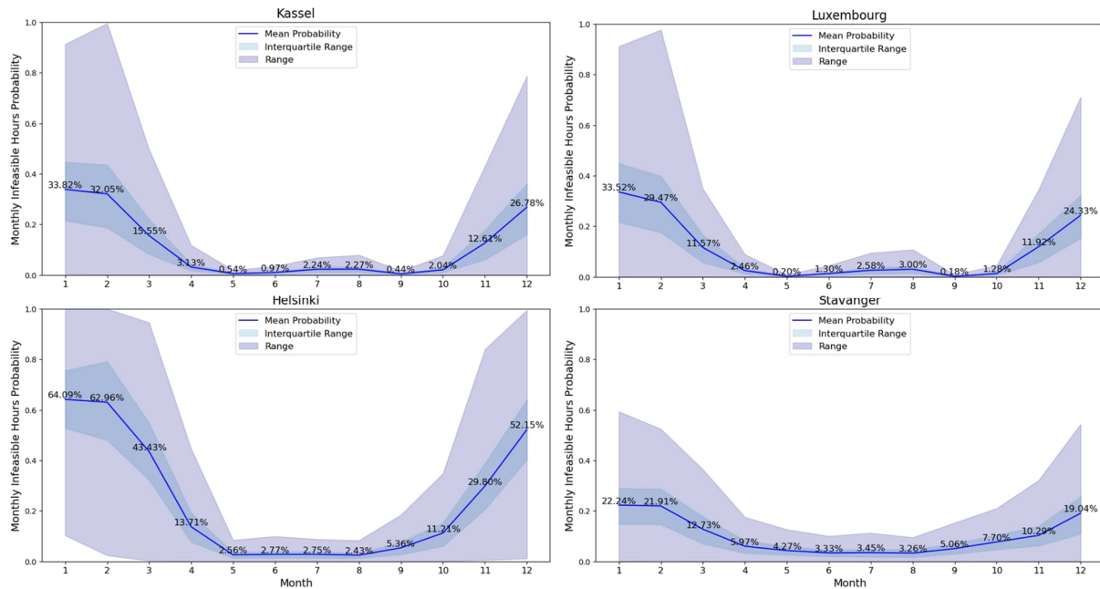
Figure 25: Monthly infeasible probabilities for operating UAS flights
