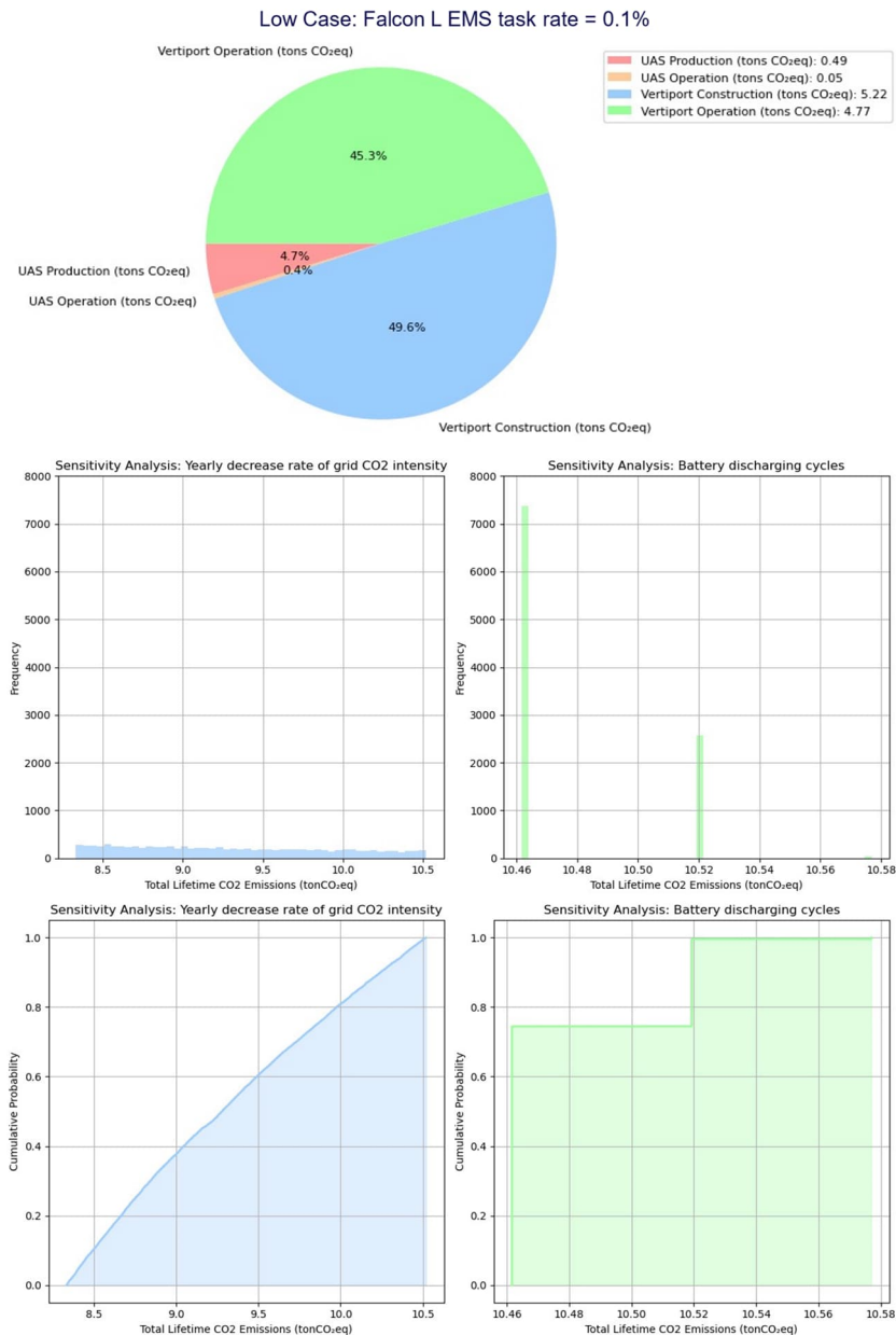
Figure 29: Low case CO 2 emission pie chart and sensitivity analysis results (Falcon L deployed in its life cycle for emergency medical services in Helsinki)
