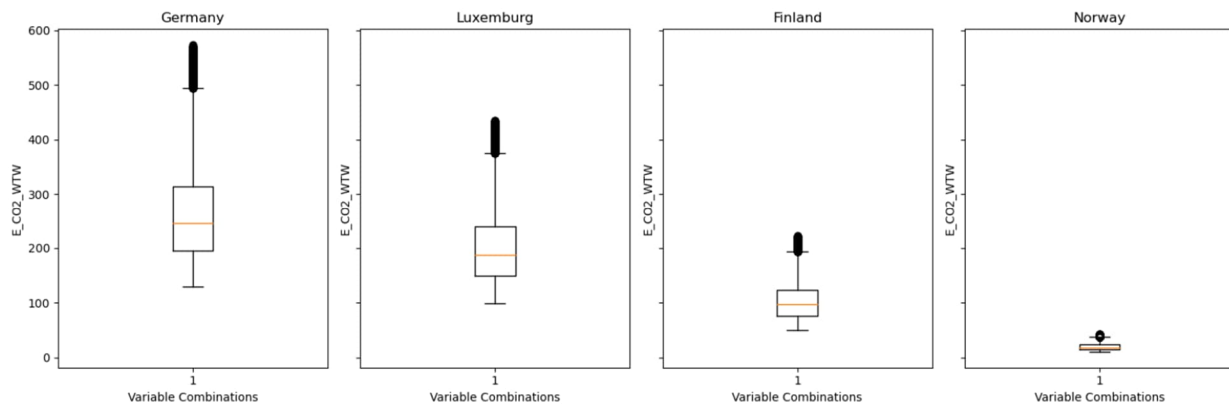
Figure 21: Statistical distribution of WTW CO 2 emission values of EH216 for each country
