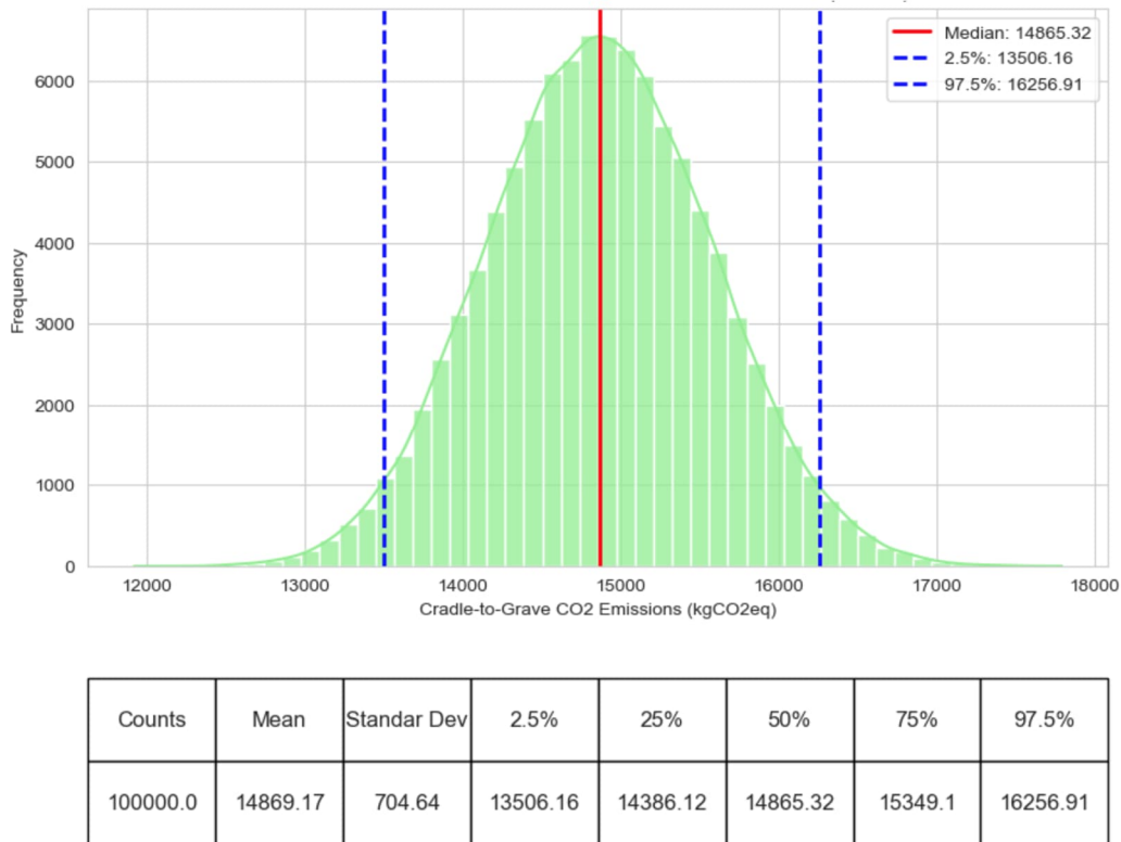
Figure 13: Result distributions of Cradle-to-Grave CO 2 emissions (EH216)
