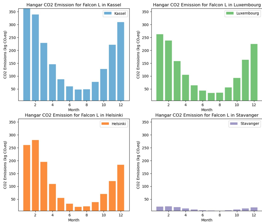
Figure 23: Hangar monthly operation CO 2 emissions for targeted cities (Falcon L)
