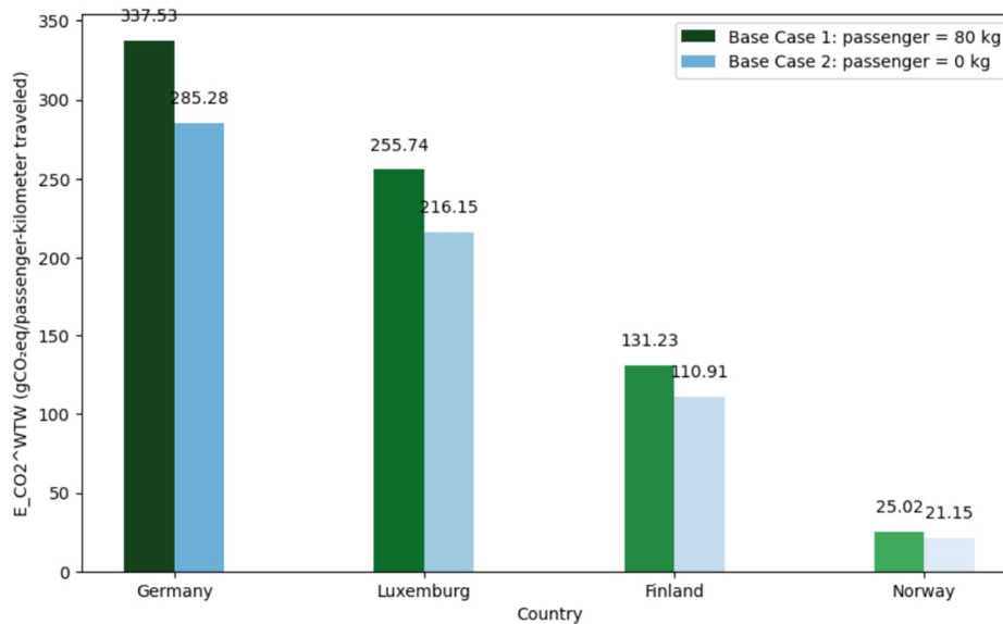
Figure 19 Base cases: Well-To-Wheel CO 2 emissions in different regions (EH216)
