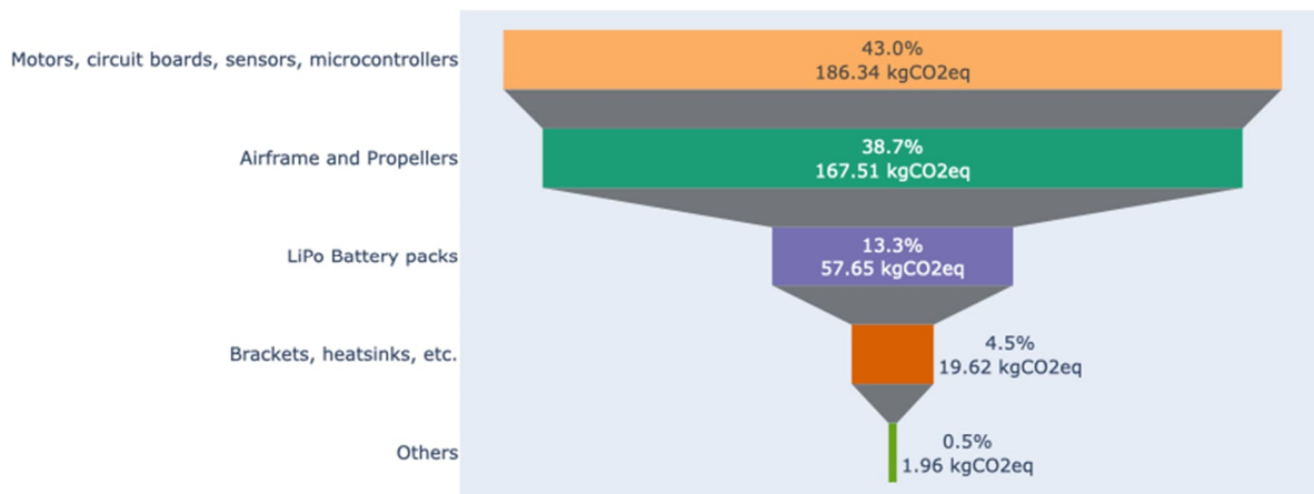
Figure 12: Percentage contributions to total Cradle-to-Grave CO 2 emissions (Falcon L)
