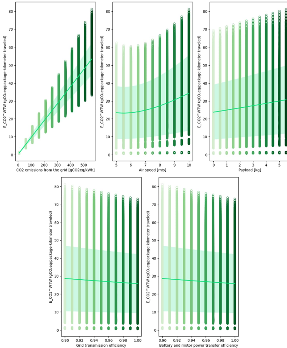
Figure 17: Well-To-Wheel CO 2 emissions of the Falcon L vary as different input variables
