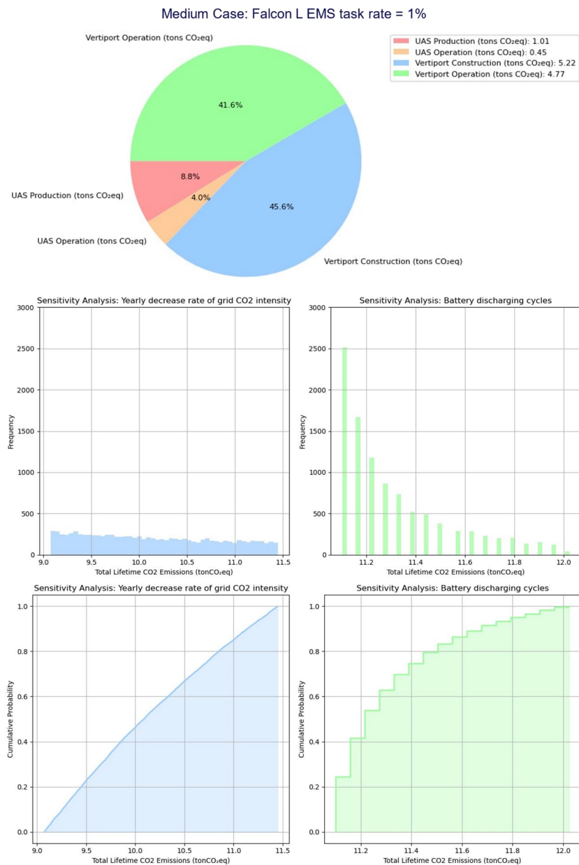
Figure 28: Medium case CO 2 emission pie chart and sensitivity analysis results (Falcon L deployed in its life cycle for emergency medical services in Helsinki)
