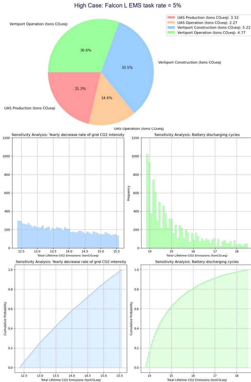
Figure 27: High case CO 2 emission pie chart and sensitivity analysis results (Falcon L deployed in its life cycle for emergency medical services in Helsinki)
