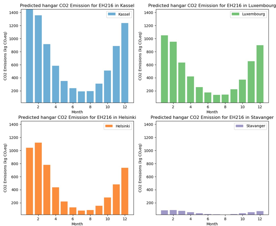
Figure 24: Hangar monthly operation CO 2 emissions for targeted cities (EH216)
