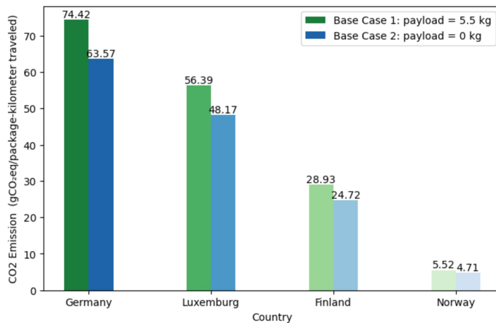
Figure 16 Base cases: Well-To-Wheel CO 2 emissions in different regions (Falcon L)
