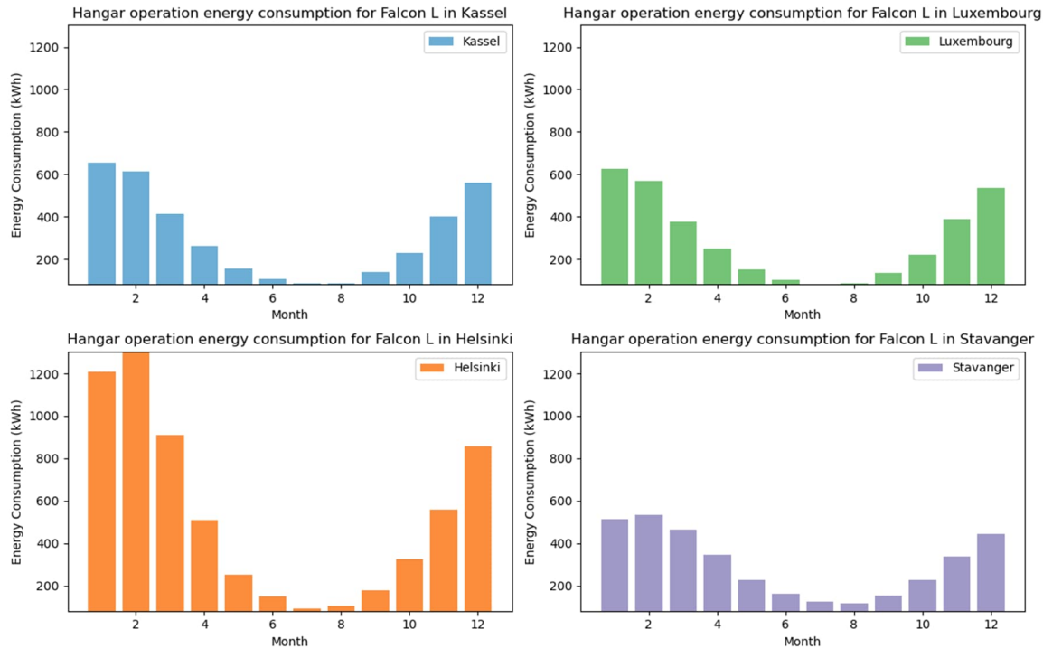
Figure 22: Predicted Falcon L's hangar operation energy consumption for targeted cities
