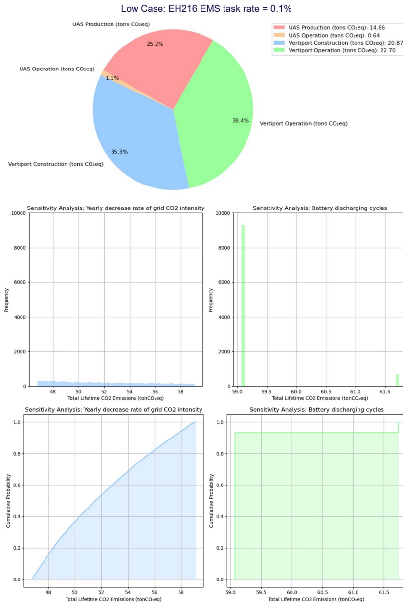
Figure 33: Low case CO 2 emission pie chart and sensitivity analysis results (EH216 deployed in its life cycle for emergency medical services in Helsinki)
