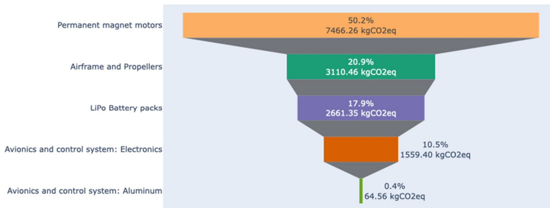
Figure 14: Expected percentage contributions to total Cradle-to-Grave CO 2 emissions (EH216)
